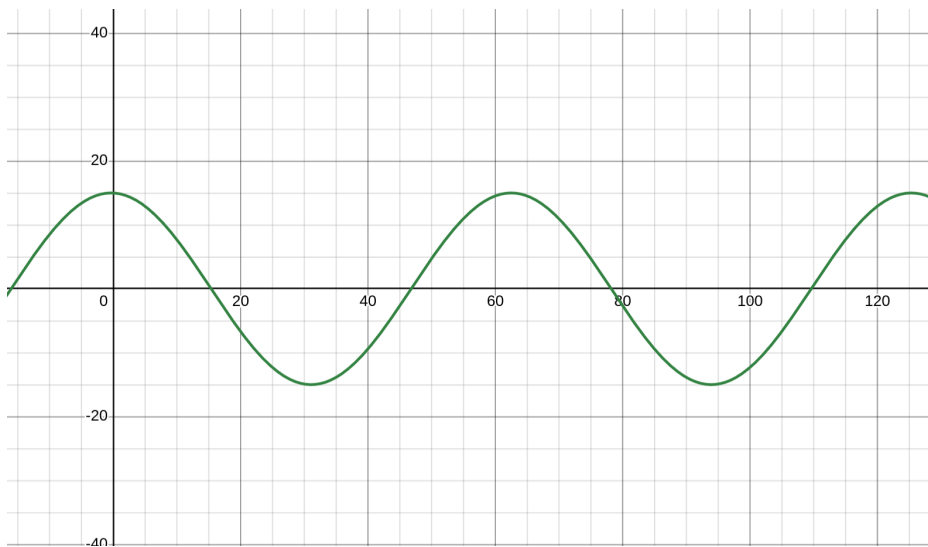
Figure 16: The plane wave at a later time, has moved to the right
