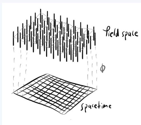
Figure 11: A representation of a 1D field space existing over a 2D space-time
