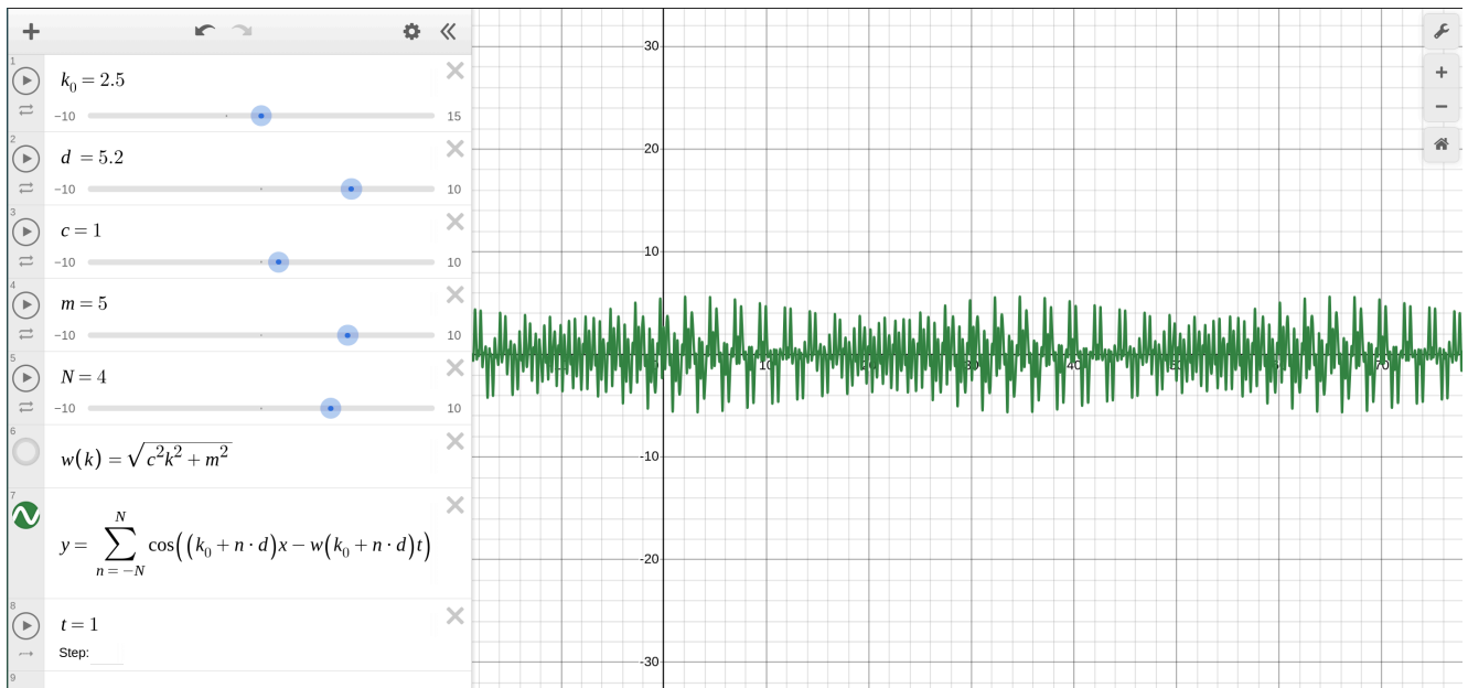
Figure 18: The waveform at t = 1 , the wave-packet is lot more dispersed as compared to its initial state
