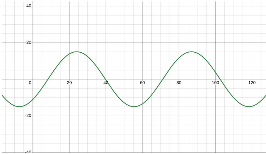
Figure 15: Initial position of a plane wave
