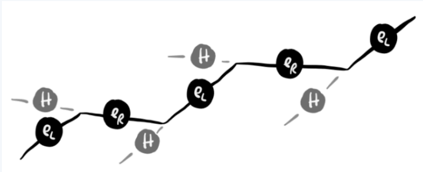
Figure 21: Oscillations from left to right chiral spinors when interacting with the Higgs field
