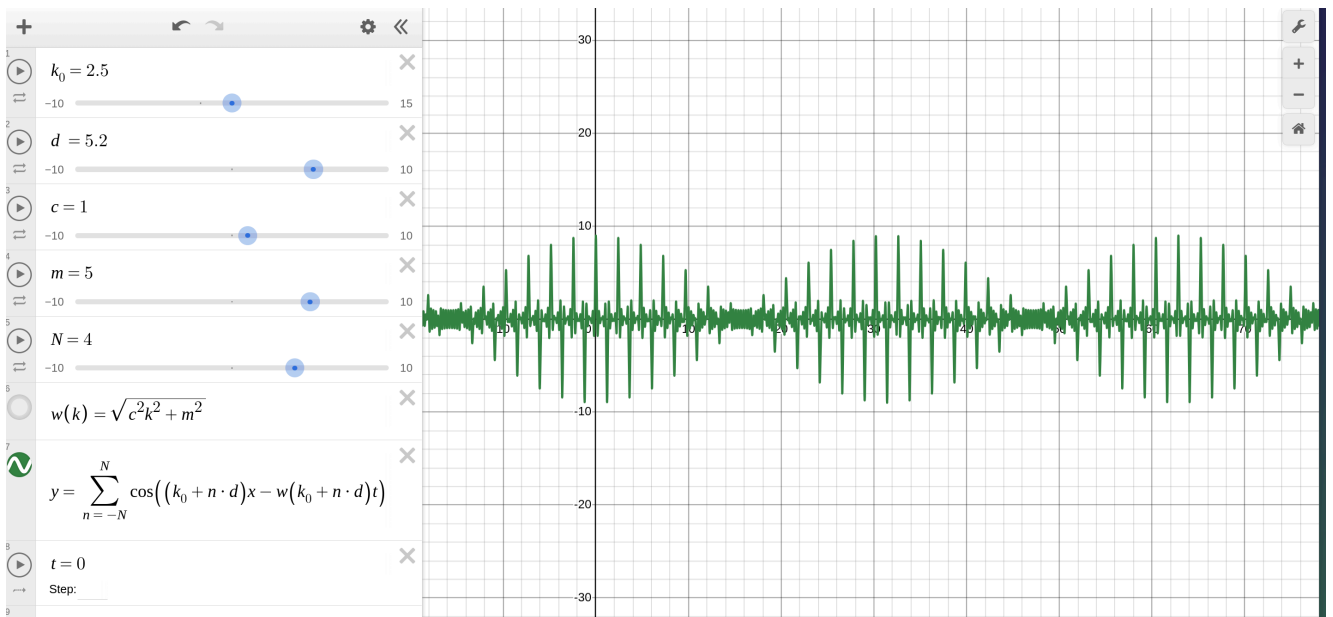
Figure 17: The waveform at t = 0
