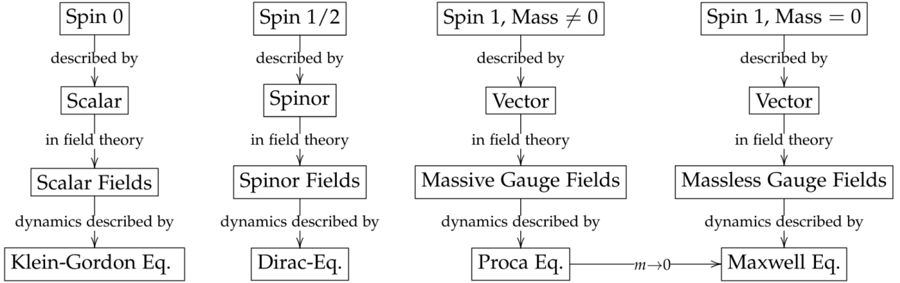
Figure 19: Free Fields discussed in this chapter
