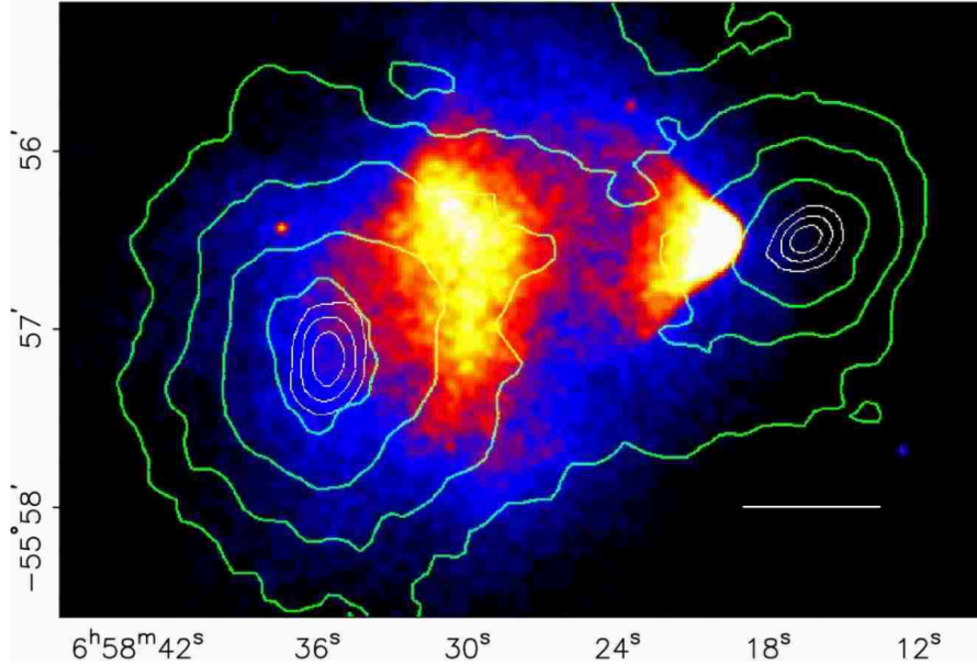
Figure 5: Bullet Cluster observations: A pair of galaxies that collided is shown here where the colors correspond to the intensity of X-rays and the contours show the estimated mass distribution obtained from weak lensing
