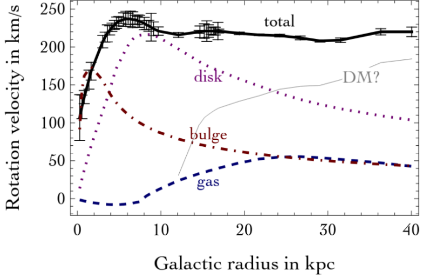
Figure 4: Velocity distribution curve along with the different components of the galaxy
