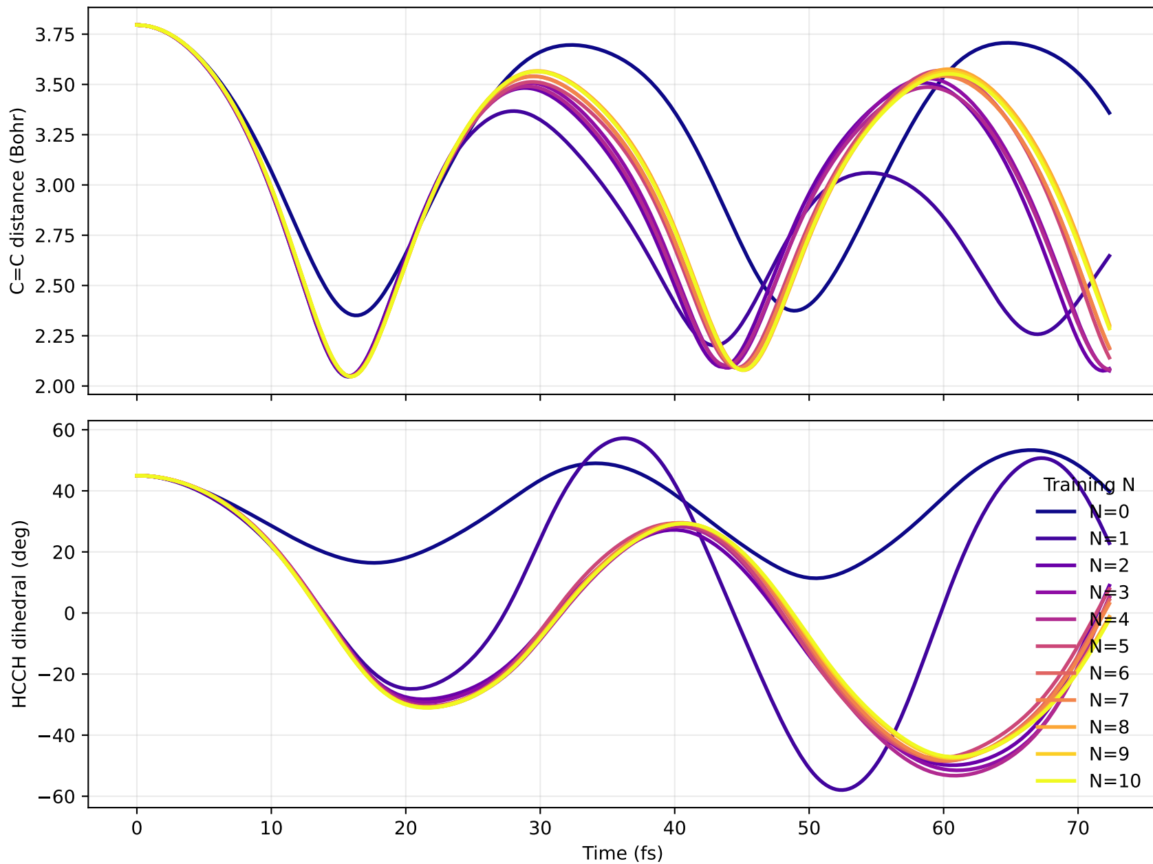
Ethene torsion run: C=C distance and HCCH dihedral
