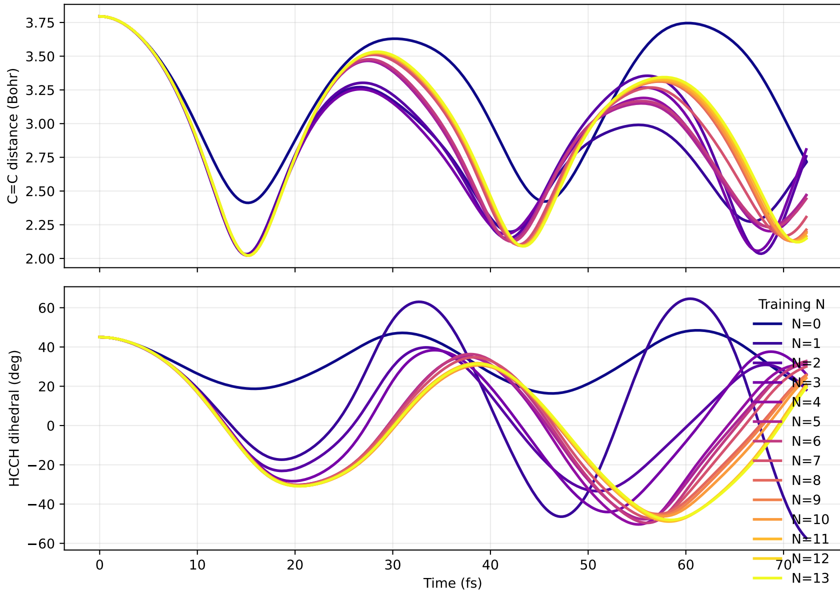
Ethene torsion run: C=C distance and HCCH dihedral
