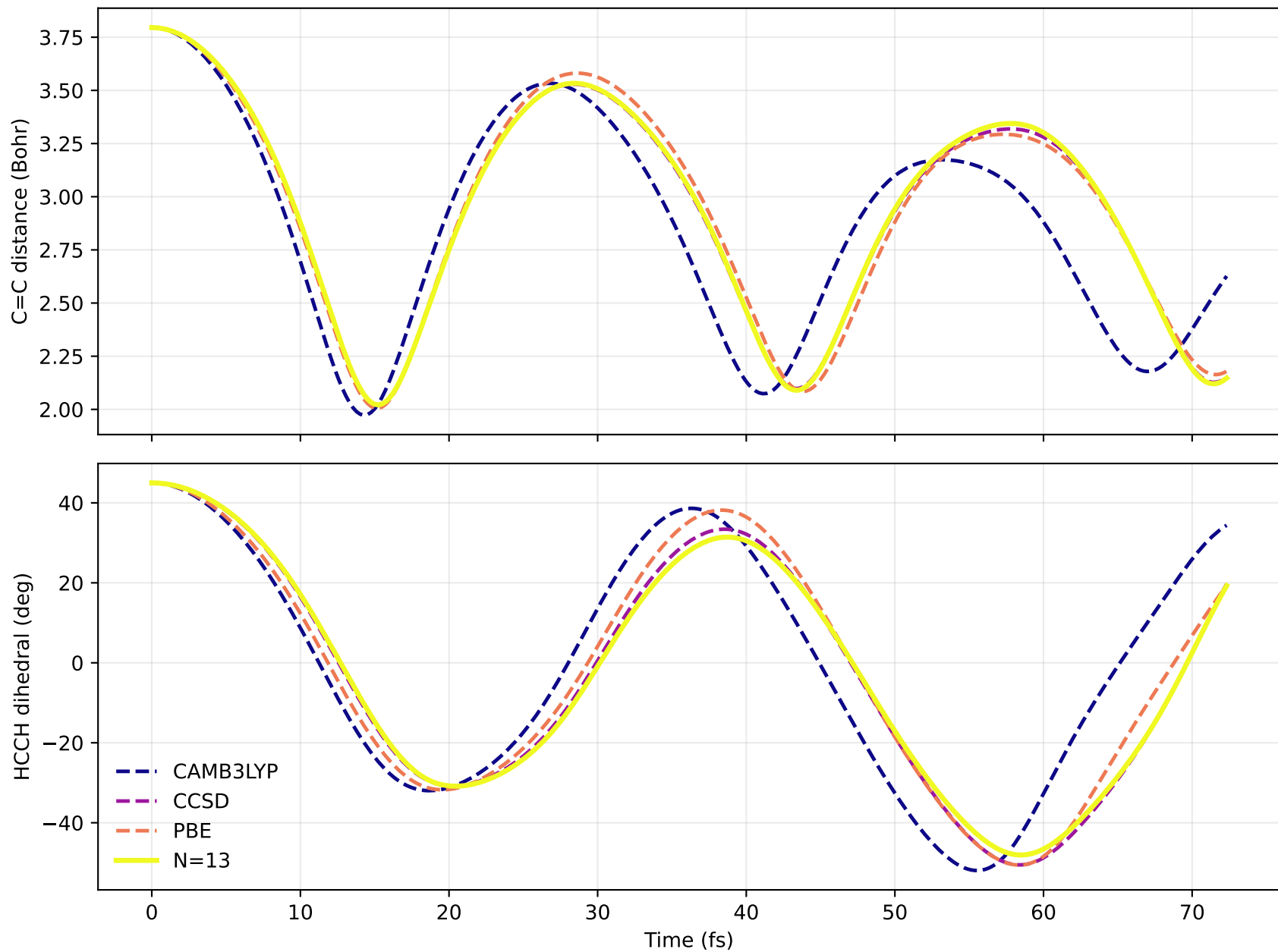
Ethene torsion run: REF vs EVCont
