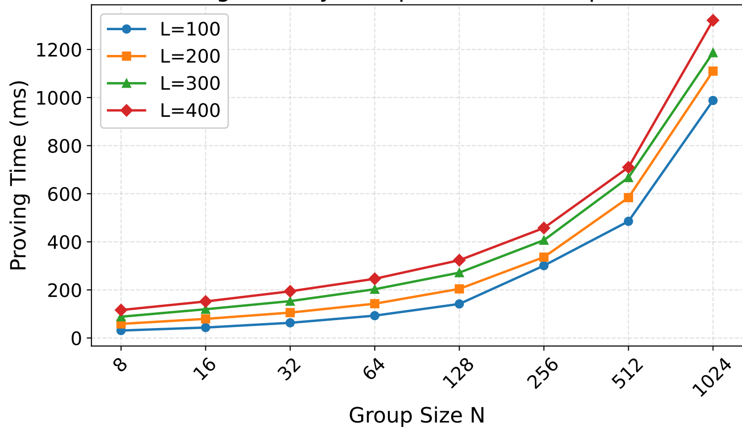
ASC-CRS Proving Time by Group Size (one line per verifier count)
