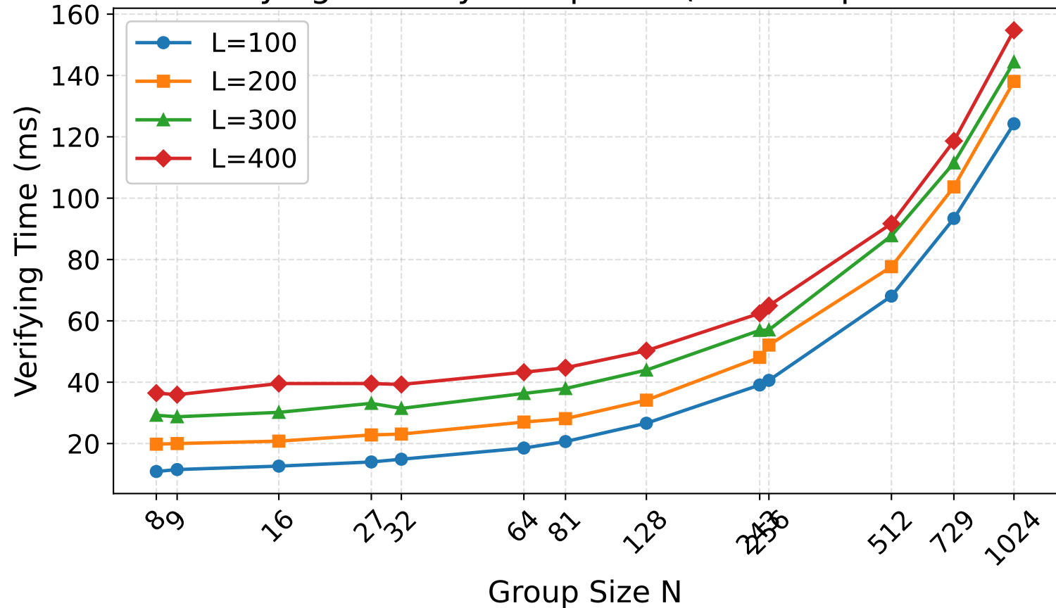
ASC-CRS Verifying Time by Group Size (one line per verifier count)
