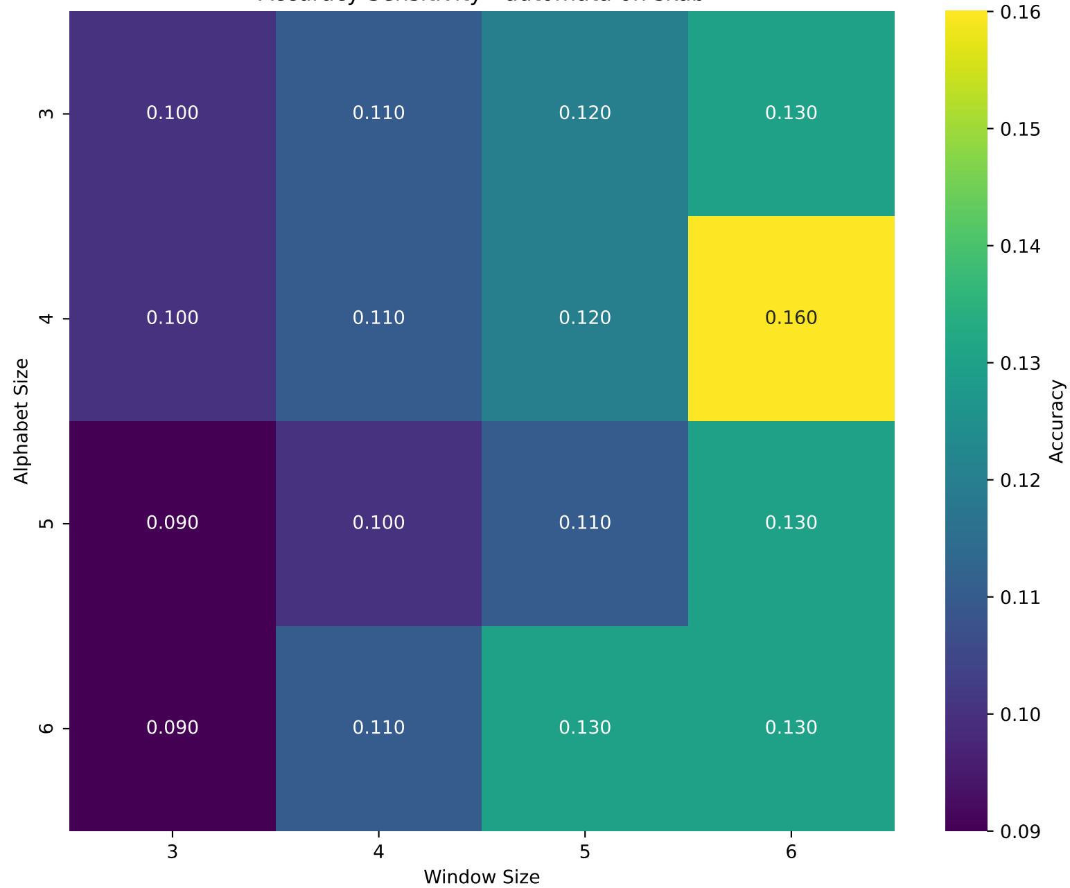
Accuracy Sensitivity - automata on skab
