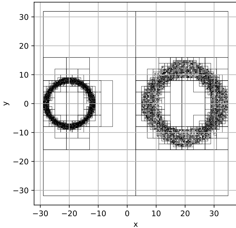
Bounding boxes del quadtree
