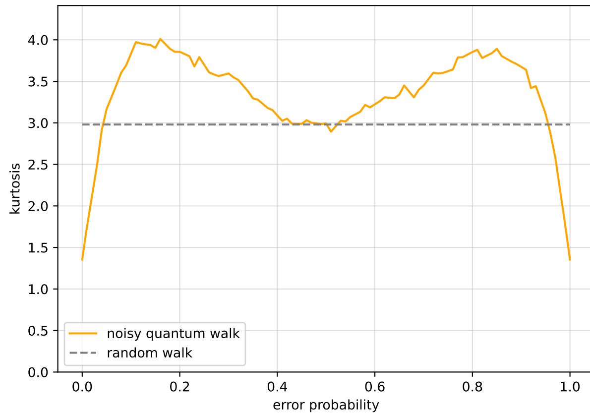
noisy quantum walk - error type: Z
