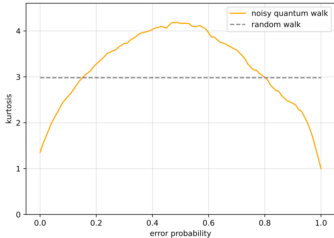
noisy quantum walk - error type: H
