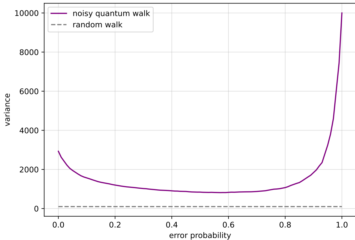
noisy quantum walk - error type: H
