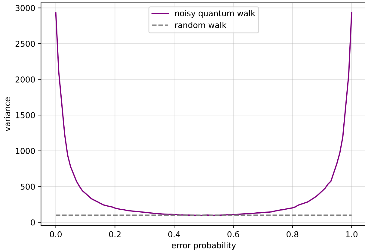
noisy quantum walk - error type: Z
