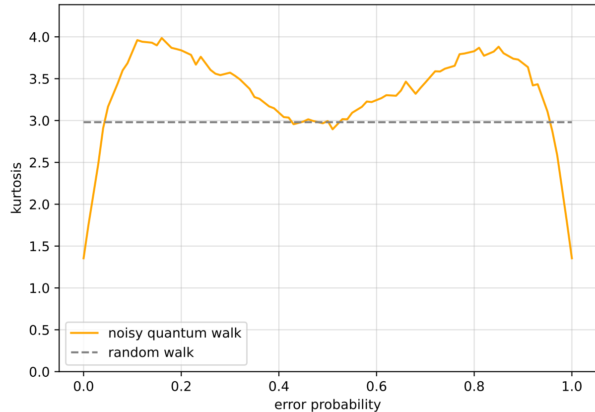
noisy quantum walk - error type: X
