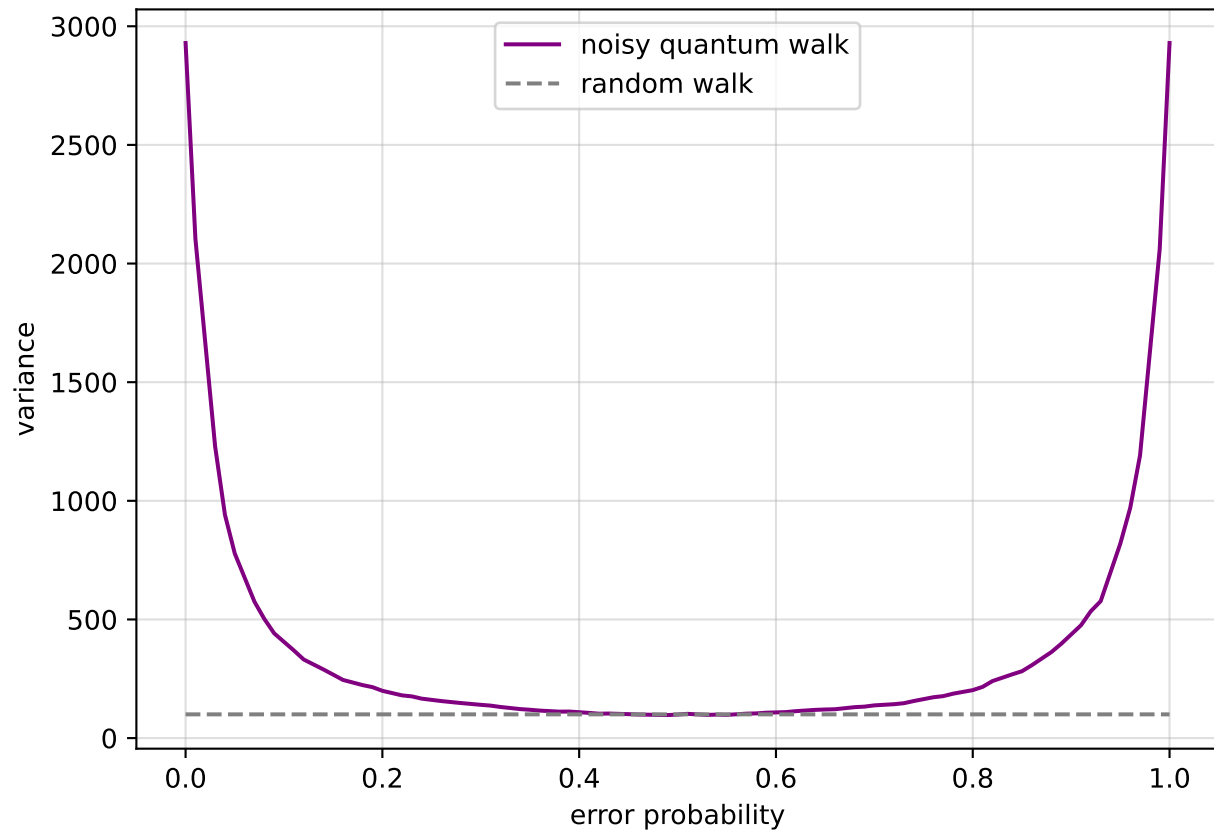
noisy quantum walk - error type: X
