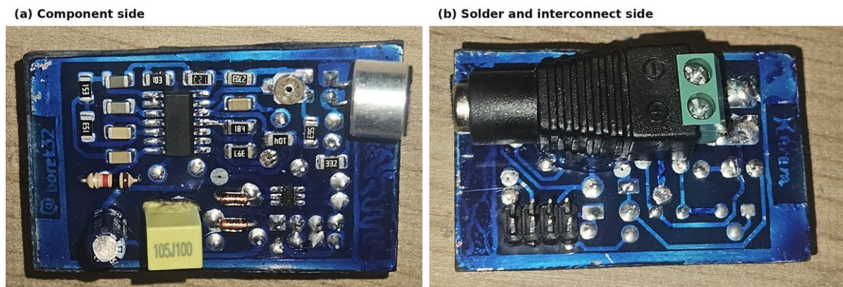
Figure 79. Final populated home-fabricated microphone and ADC PCB: (a) component side; (b) solder and interconnect side.
