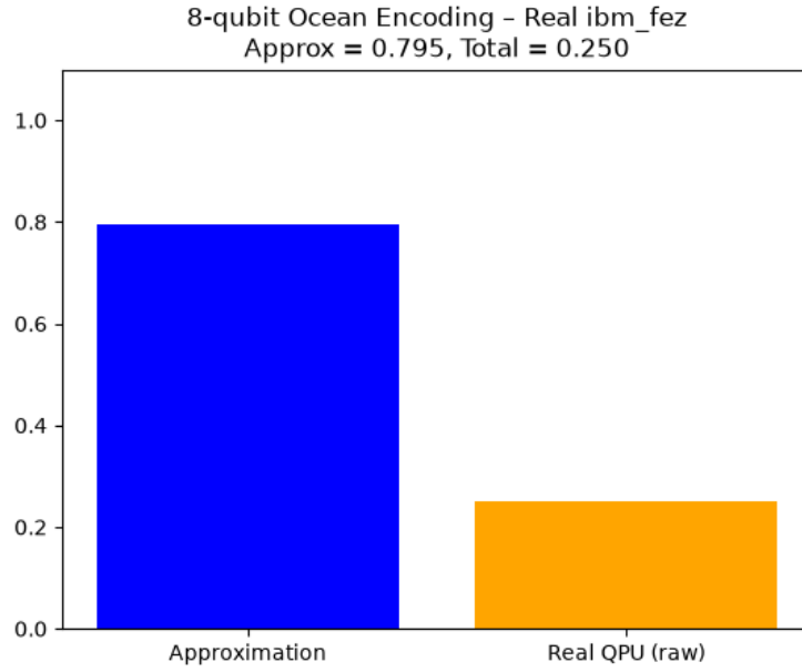
Figure 4: Real-hardware fidelity for the 8-qubit variational encoding: approximation fidelity F_{\text{approx}} = 0.795 ; measured hardware fidelity F_H = 0.25 .
