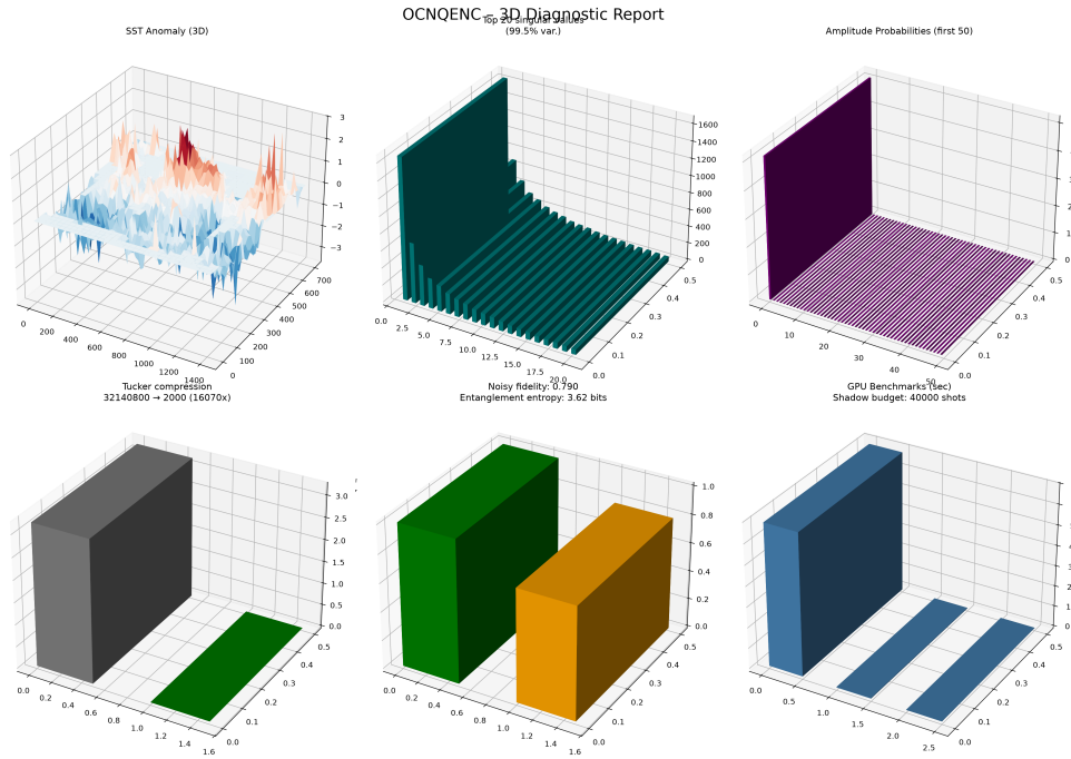
Figure 2: Three-dimensional visualisation of the SST anomaly field, singular values, amplitude probabilities, Tucker compression, noise fidelity, and GPU benchmarks.
