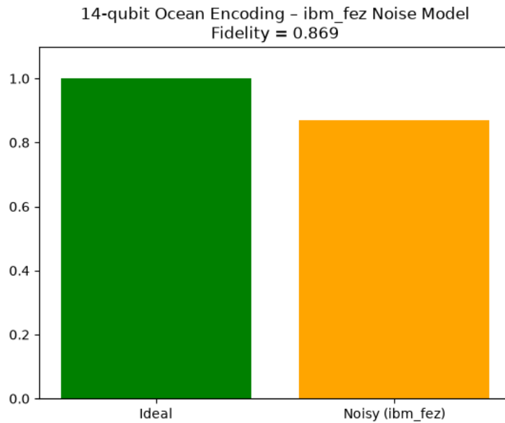
Figure 3: Simulated fidelity under the calibration-derived noise model for the 14-qubit exact encoding ( F_H = 0.869 ).
