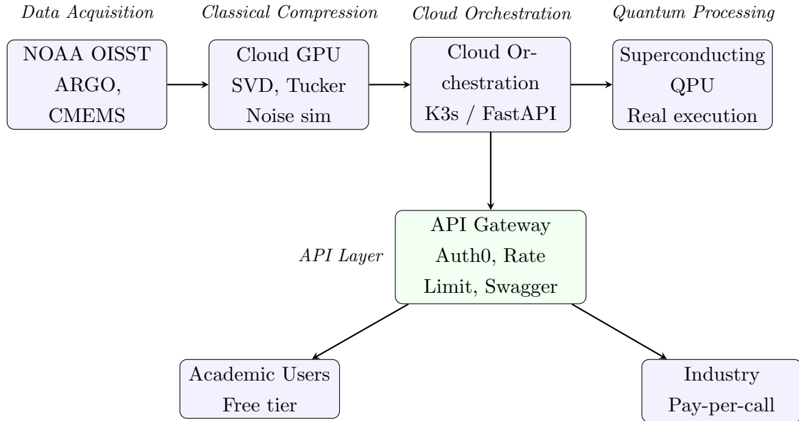
Figure 5: Architecture of the quantum ocean encoding API. The pipeline flows from NOAA data acquisition through GPU compression and cloud orchestration to QPU execution, exposed to users via a managed API gateway.
