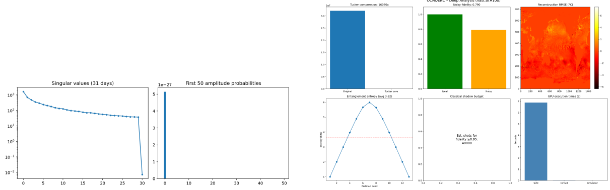
Figure 1: Singular-value spectrum and encoding diagnostics. (a) Singular values of the 31-day SST SVD and the first 50 amplitude probabilities. (b) Six-panel diagnostic report: Tucker compression, noisy fidelity, RMSE map, entanglement entropy, shadow budget, and GPU benchmarks.
