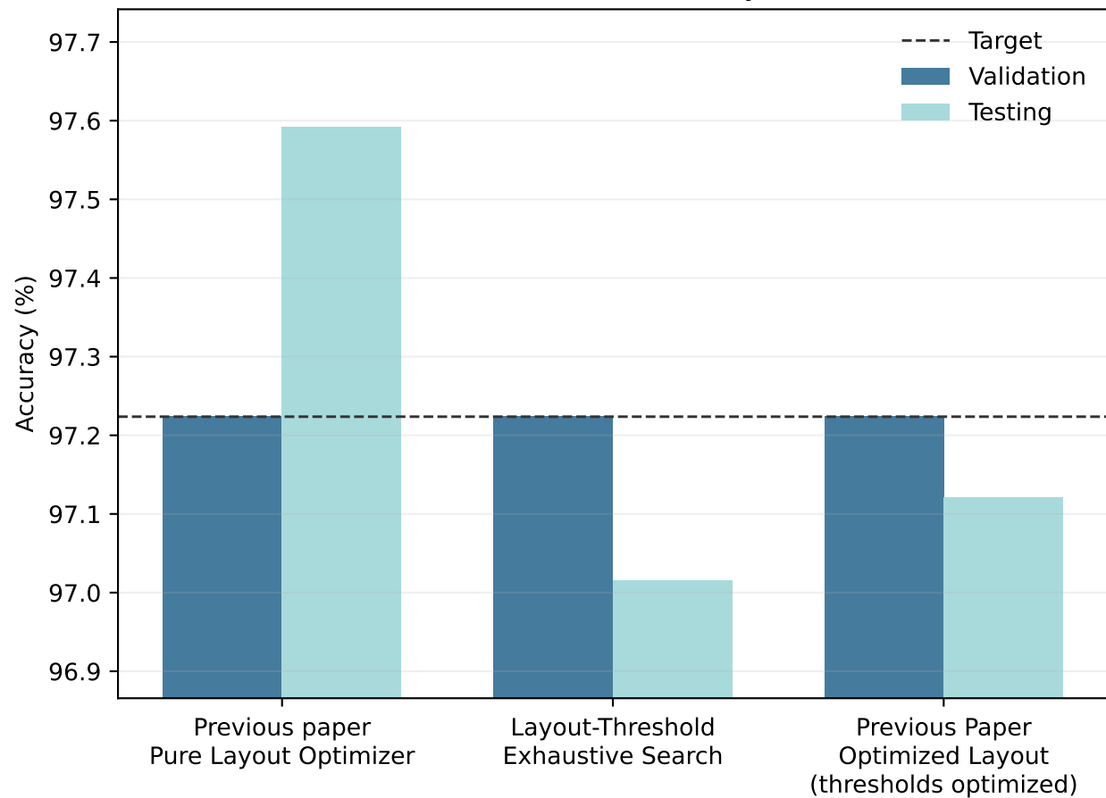
End-to-end accuracy
