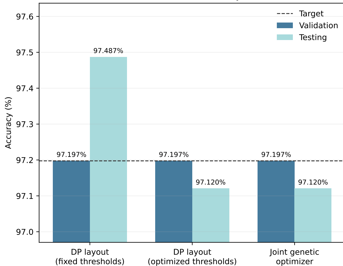
End-to-end accuracy
