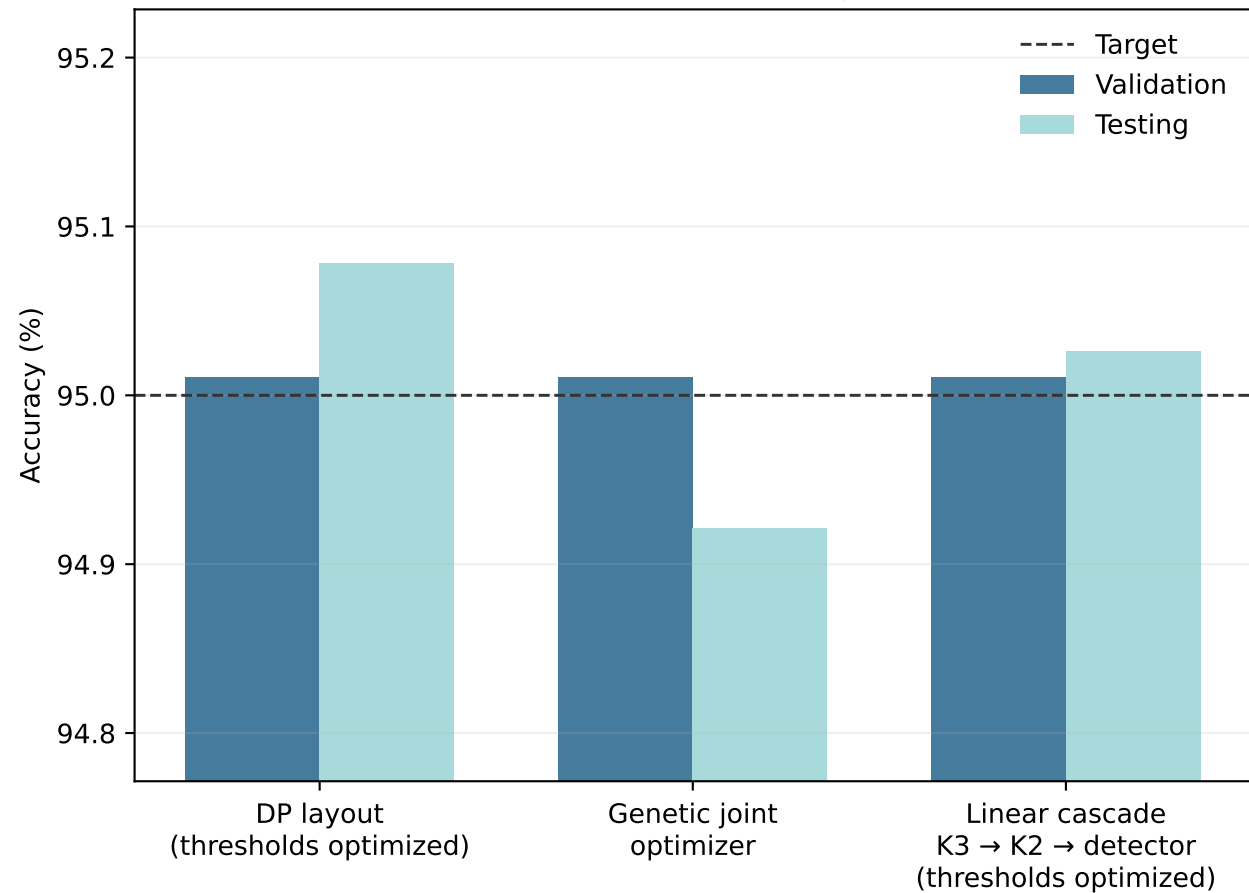
End-to-end accuracy
