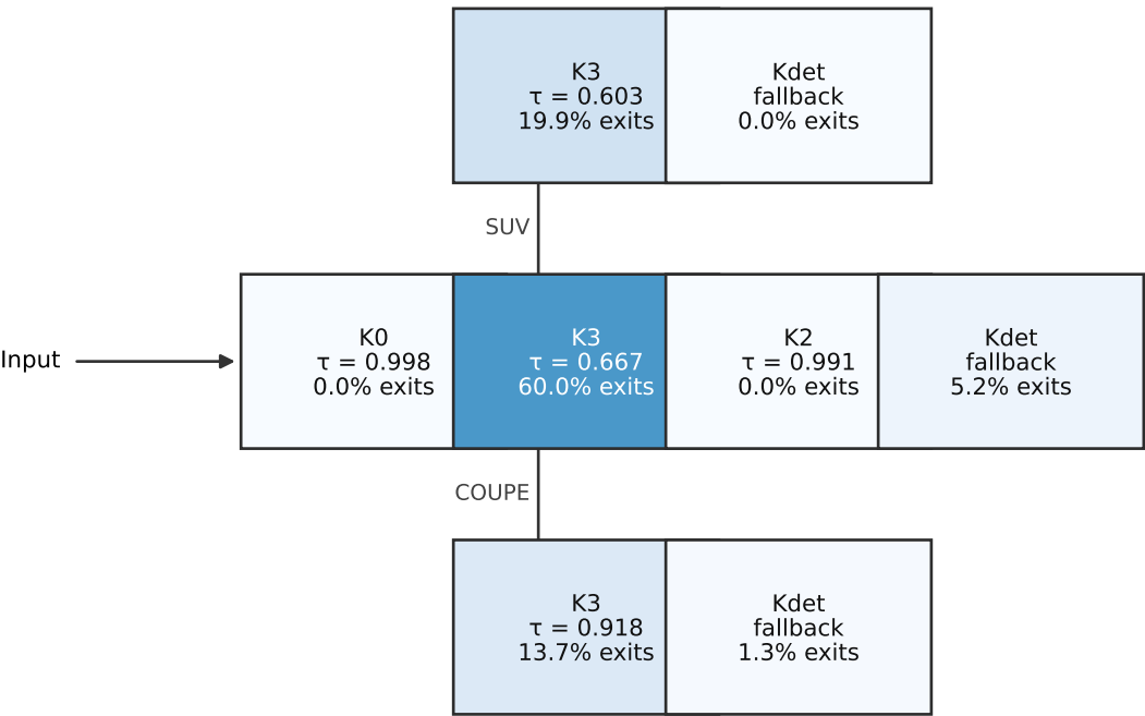
Brute force (0.9662) 660.1 ms · 96.06% accuracy
