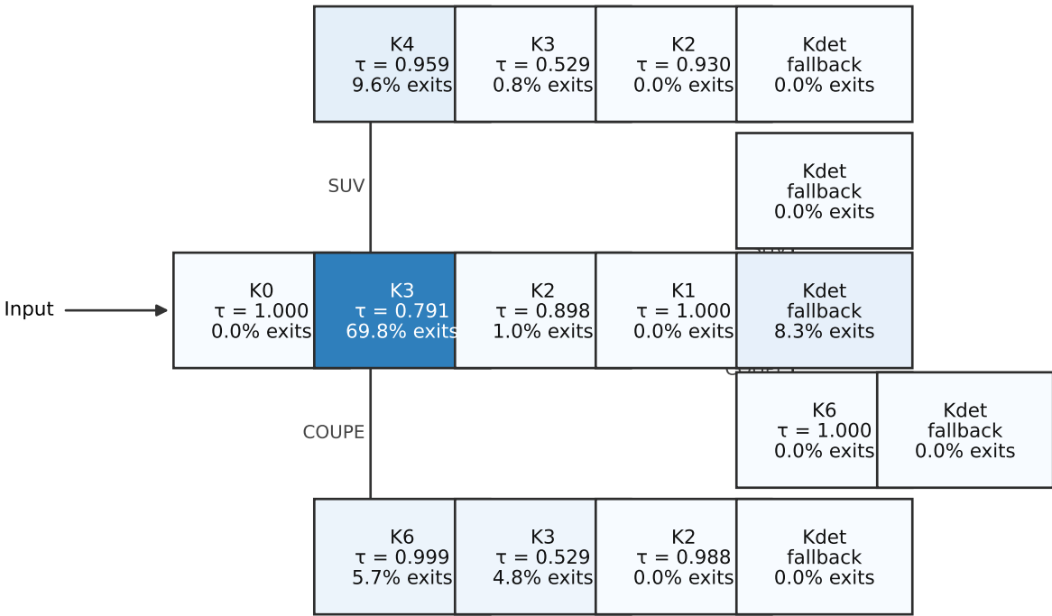
Brute force (0.9662) 660.1 ms · 96.06% accuracy
