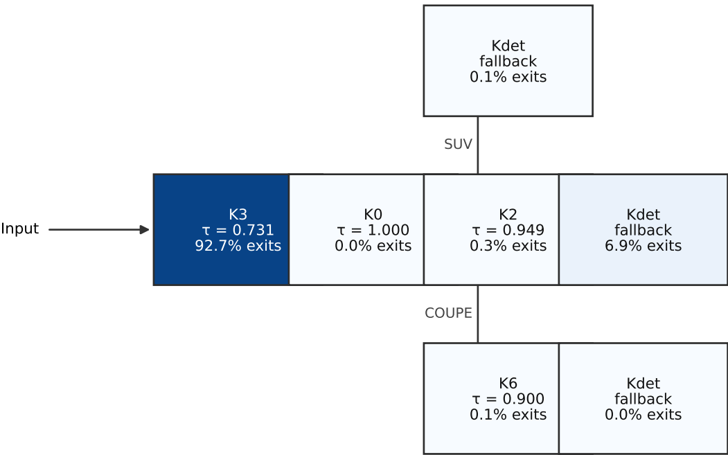
Approx. joint (0.9662) 710.1 ms · 96.71% accuracy
