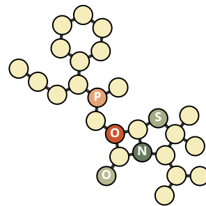
Azidocillin
