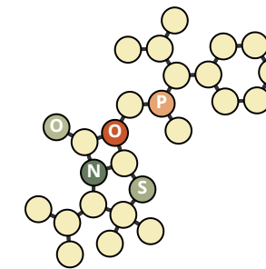
Carbenicillin
