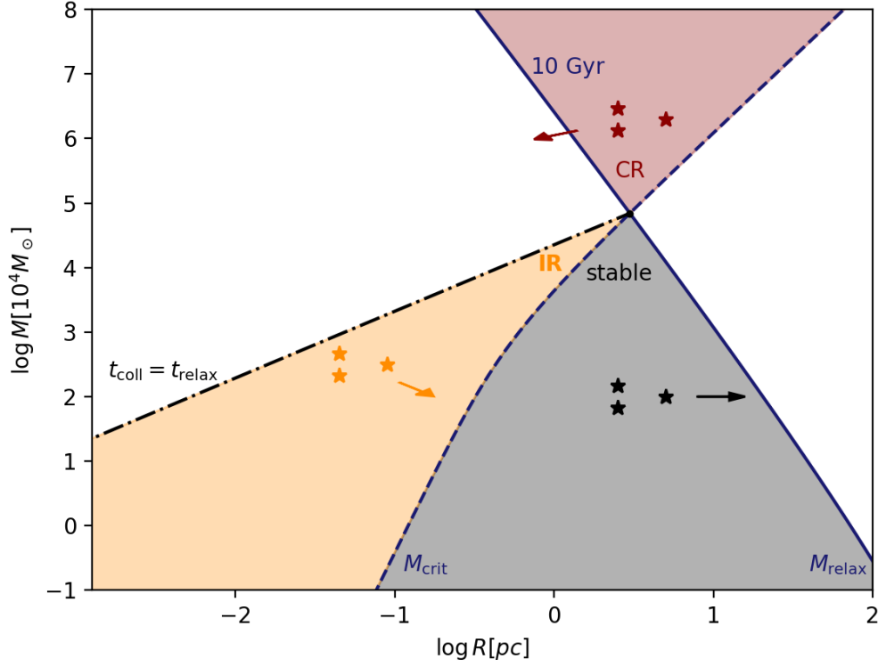
Figure 2.1: Collision and relaxation timescales in a mass versus radius diagram. Dashed line correspond to the critical mass M_{\text{crit}} , while solid line correspond to the relaxation mass M_{\text{relax}} , both calculated for solar-mass clusters, characteristic time t_H = 10^{10} yr and q = 0 . The black dash-dotted line represents t_{\text{coll}} = t_{\text{relax}} , with t_H varying from 10^2 yr to 10^{10} yr and q = 0 . Clusters above the black dash-dotted line satisfy t_{\text{coll}} \leq t_{\text{relax}} . The collisional regime (CR) is defined by t_{\text{coll}} \leq t_H \leq t_{\text{relax}} (red colored zone); the stable regime is where t_{\text{relax}} \leq t_H \leq t_{\text{coll}} (gray colored zone); and the intermediate regime (IR) fulfils t_{\text{relax}} \leq t_{\text{coll}} \leq t_H (orange colored zone). The arrows point toward the predicted movements in the M–R diagram.
