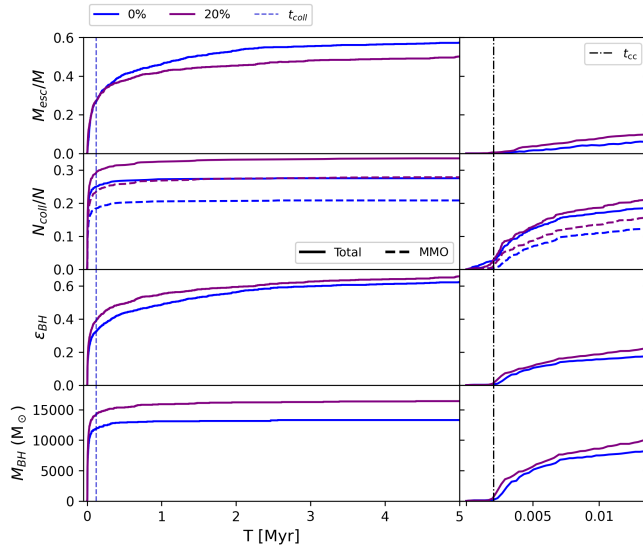
Fig. 3: Mass components and \epsilon_{\text{BH}} evolution over time of stars. Blue curves are for A_0 , and purple for A_{20} . Top panel is for escaped mass normalized by the total stellar mass. Second panel shows collisions normalized by the initial number of stars, where solid lines are for the total and dashed lines for collisions involving the most massive object. Third panel shows \epsilon_{\text{BH}} (Eq. 14), and bottom panel shows the mass of the most massive object. Left column is for 5 Myr, with the vertical blue dashed line representing t_{\text{coll}} . Right column is a zoom to 40 relaxation times ( \sim 0.014 Myr), where the dot-dashed black line is the mean core collapse time.
