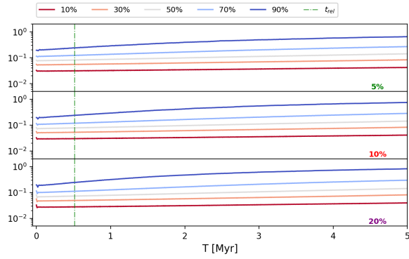
Fig. E.2: Lagrangian radii for gas of three variants of Model N. Top panel is for N_5 , middle is for N_{10} and bottom panel is for N_{20} . Left column shows the full simulation time (5 Myr) while right column shows the evolution until 40 relaxation times.
