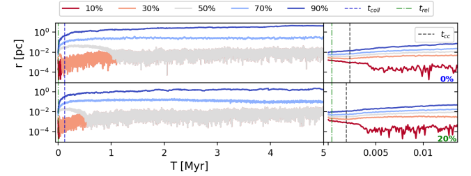
Fig. 2: Lagrangian radii for stars, from 10% (red) to 90% (blue). The top panel corresponds to A_0 , and bottom panel to A_{20} . The left column shows the full simulation time (5 Myr), while the right column shows the evolution up to 40 relaxation times. Blue dashed and green dot-dashed lines are the initial collision and relaxation timescales, respectively. Black dot-dashed lines are the core collapse.
