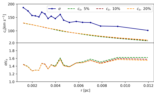
Fig. E.3: Sound speed of gas ( c_s ) and velocity dispersion ( \sigma ) for family A models.
