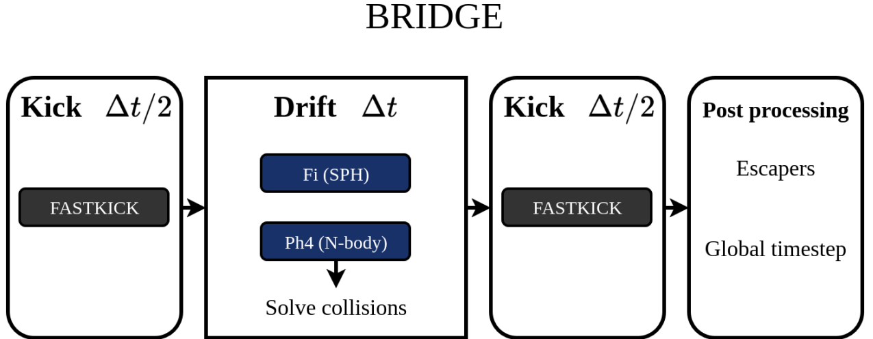
Figure 3.5: Scheme of the BRIDGE coupling strategy. In the kick steps, FAST-KICK computes the mutual gravitational forces between stars and gas, and the velocities of both components are updated. In the drift step, each code evolves its particles independently: Ph4 handles stellar dynamics (including collision detection and mergers), while Fi evolves the gas. After the kick-drift-kick cycle, the global BRIDGE time step is updated based on the gas free-fall time and the coupling timescales ( t_{\text{ff}} , \Delta t_{\text{coup,gas}} , \Delta t_{\text{coup,stars}} ). This updated timestep is used for both the next BRIDGE step and the Fi integration. Additionally, escaped N-body particles are identified and tagged in the post-processing phase.
