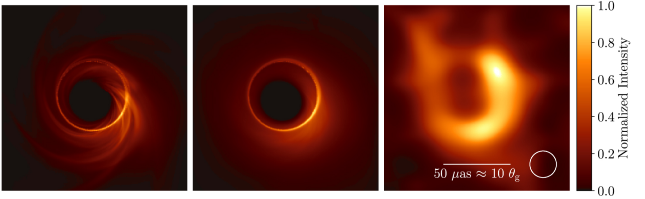
Figure 1.2: Simulated images of Sgr A * . The left panel is a snapshot of a numerical simulation of Sgr A * , and middle panel is the average of snapshots of the simulation. On the right panel, a representative image reconstruction, using the synthetic visibilities from the simulation. Credits: EHT Collaboration et al. (2022).
