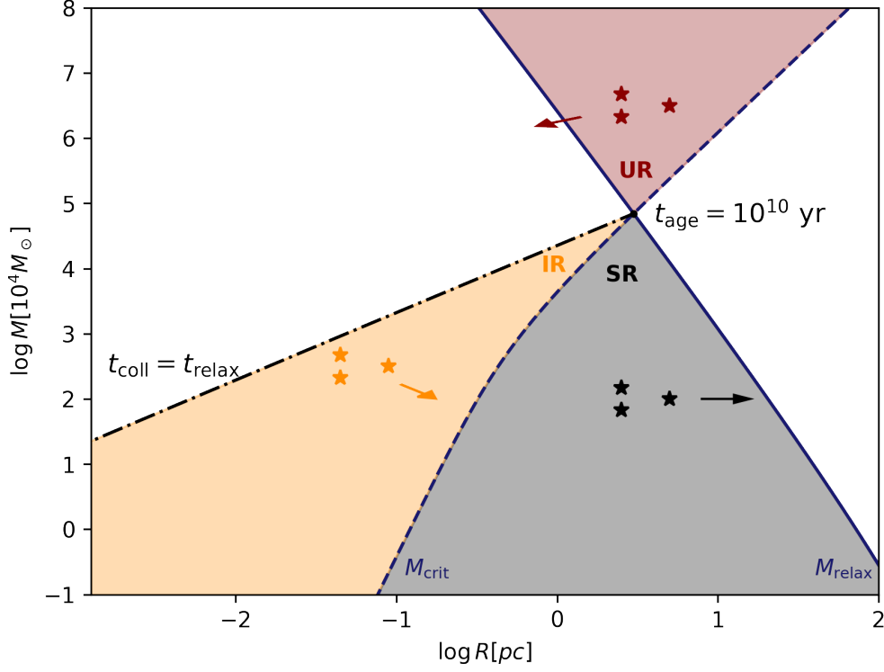
Figure 2.1: Collision and relaxation timescales in a mass versus radius diagram. The blue dashed line correspond to the critical mass M_{\text{crit}} , while blue solid line correspond to the relaxation mass M_{\text{relax}} , both calculated for clusters formed by solar mass stars, characteristic time t_H = 10^{10} yr and q = 0 . The black dash-dotted line represents t_{\text{coll}} = t_{\text{relax}} , with t_H varying from 10^2 yr to 10^{10} yr and q = 0 . Clusters above the black dash-dotted line satisfy t_{\text{coll}} \leq t_{\text{relax}} . The unstable regime (UR) is defined by t_{\text{coll}} \leq t_H \leq t_{\text{relax}} (red colored zone); the stable regime is where t_{\text{relax}} \leq t_H \leq t_{\text{coll}} (gray colored zone); and the intermediate regime (IR) fulfills t_{\text{relax}} \leq t_{\text{coll}} \leq t_H (orange colored zone). The arrows point toward the predicted movements in the M–R diagram.
