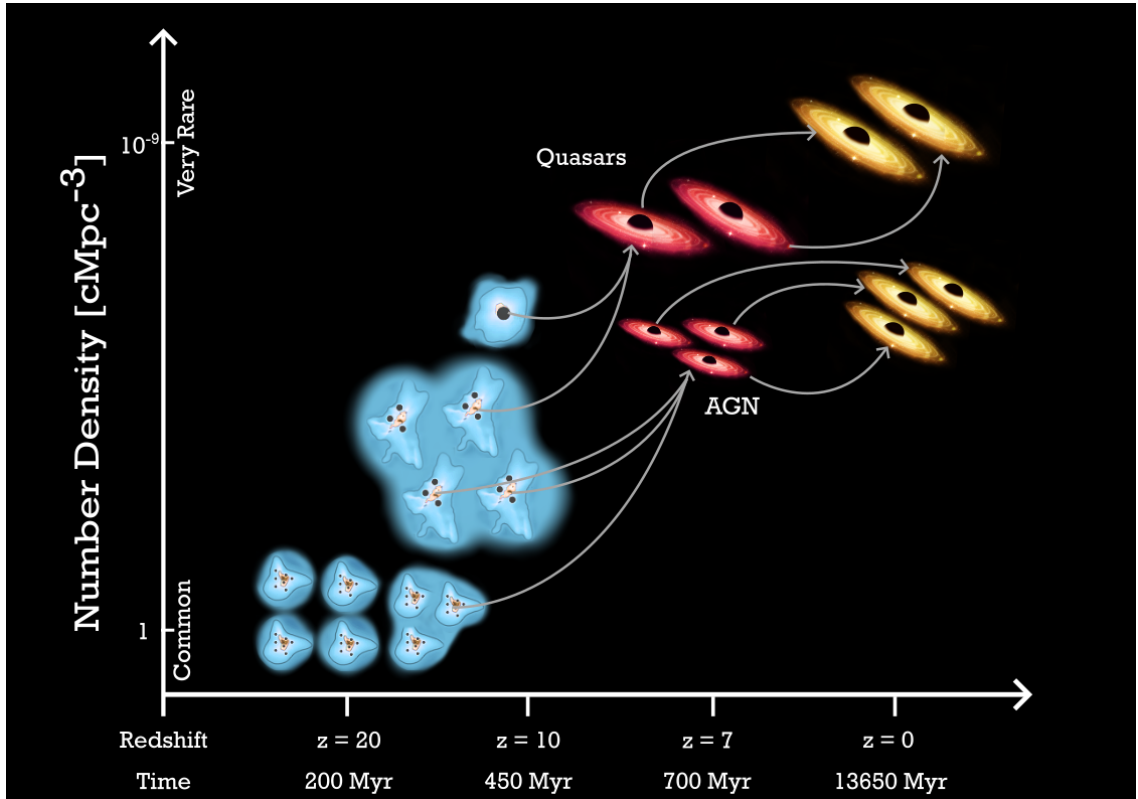
Figure 1.3: BH abundance (number density) in \text{cMpc}^{-3} (y-axis) vs redshift (x-axis). The y-axis, from top to bottom, goes from very rare ( \sim 10^{-9} ) to common \sim 1 . Credits: Regan and Volonteri (2024).
