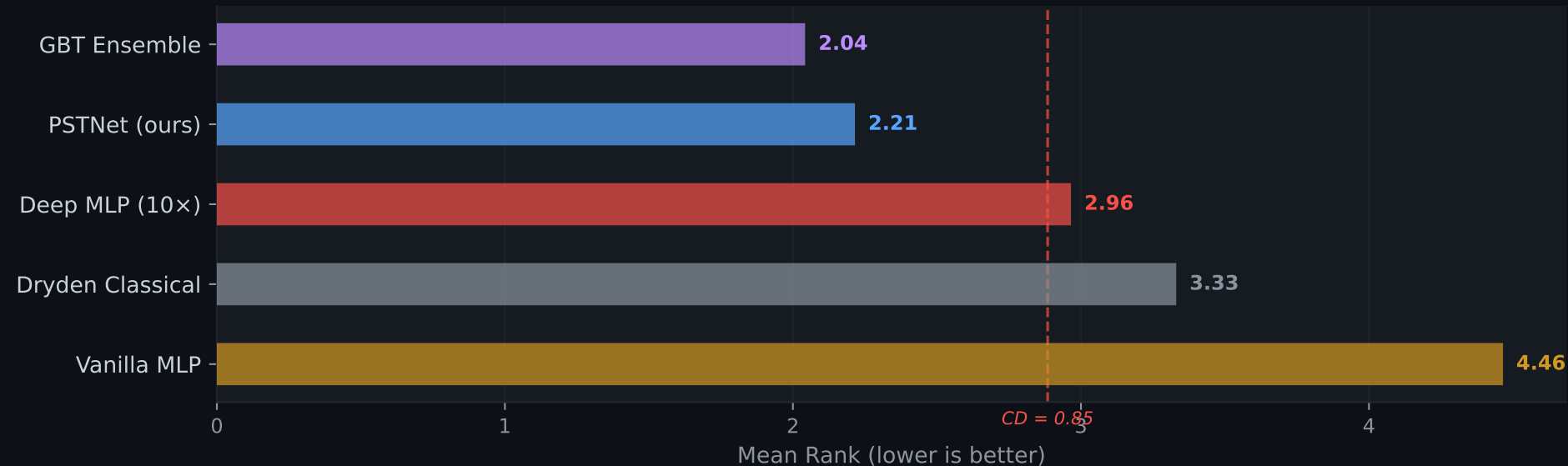
Critical Difference Diagram (Nemenyi, N=52)
