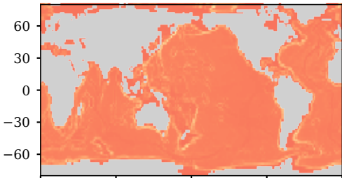
(c) NN-8 / PHYS drag ratio ( \log_{10} )
