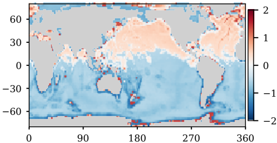
(c) NN-8 / PHYS drag ratio ( \log_{10} )
