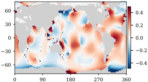
PHYS: \Delta spring range per m SLR [cm]; dots: folds disagree in sign
