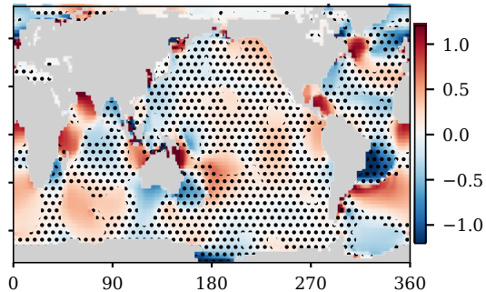
PHYS: \Delta spring range per m SLR [cm]; dots: folds disagree in sign
