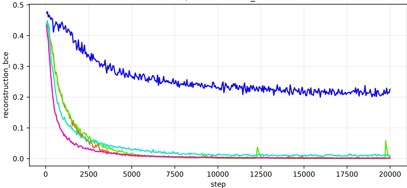
train/reconstruction_bce
