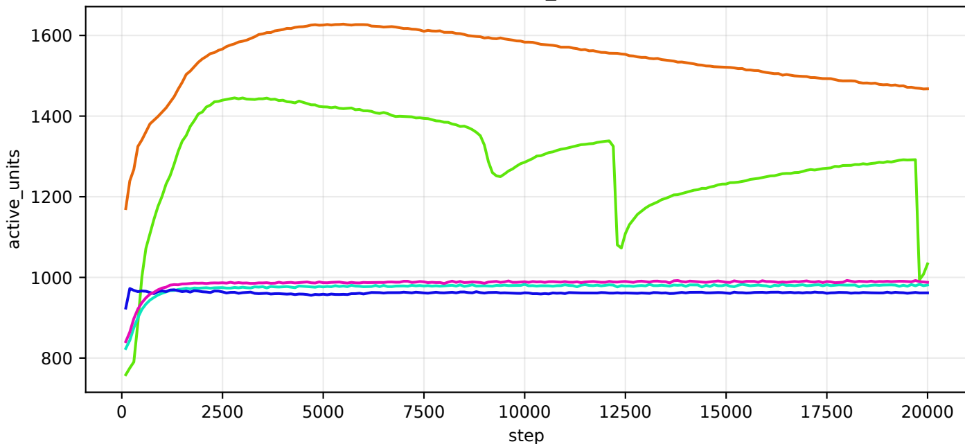
val/active_units
