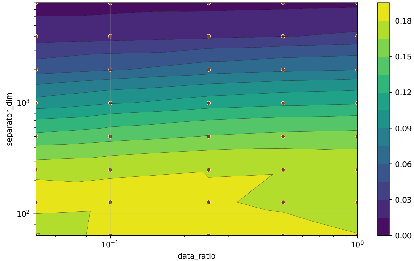
train/latent_post_hoyer (steps=all, last)
