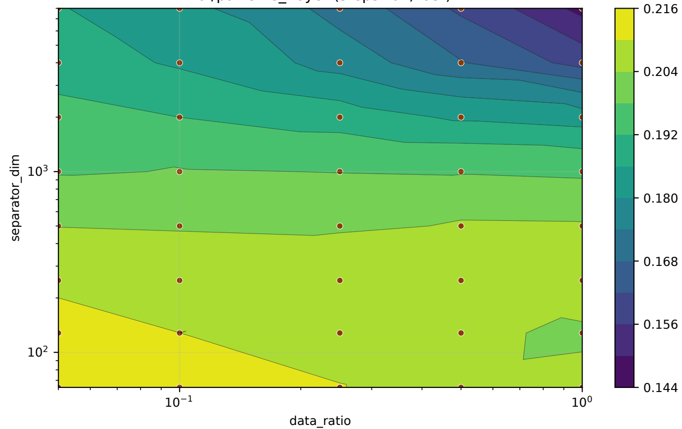
val/patterns_hoyer (steps=all, last)
