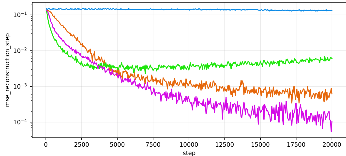
train/mse_reconstruction_step
