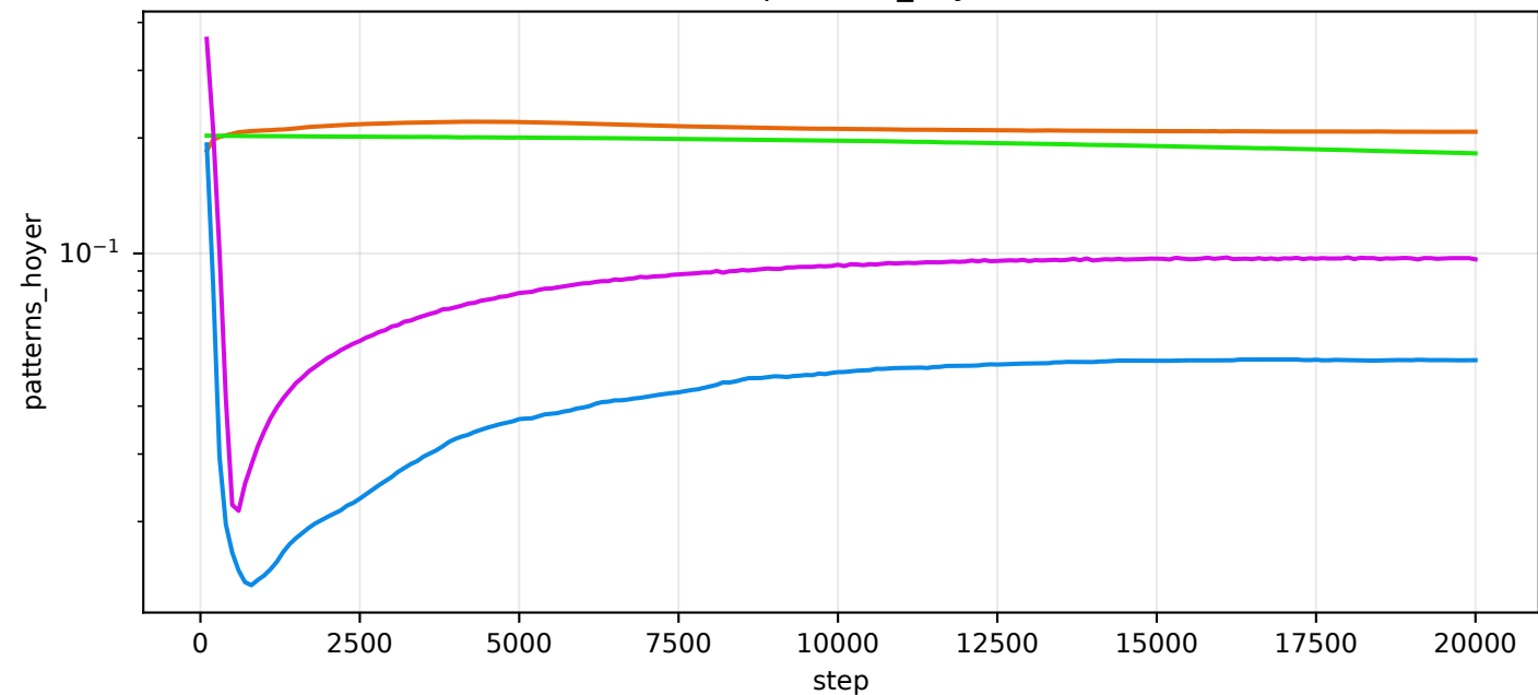
train/patterns_hoyer
