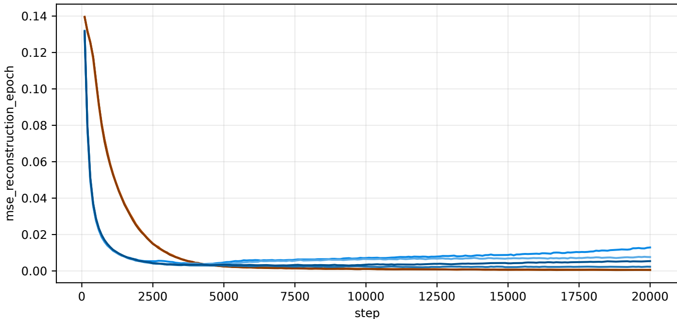
train/mse_reconstruction_epoch
