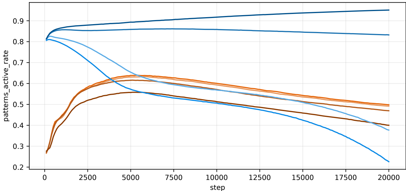
train/patterns_active_rate
