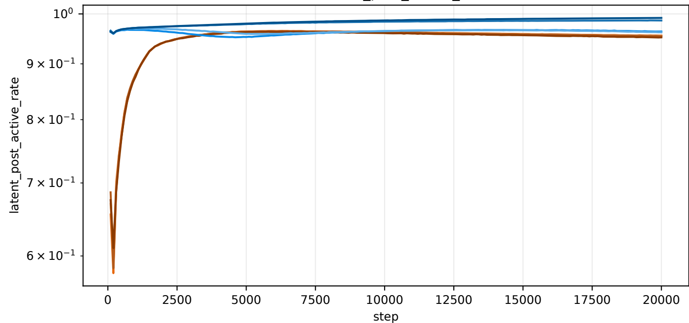
train/latent_post_active_rate
