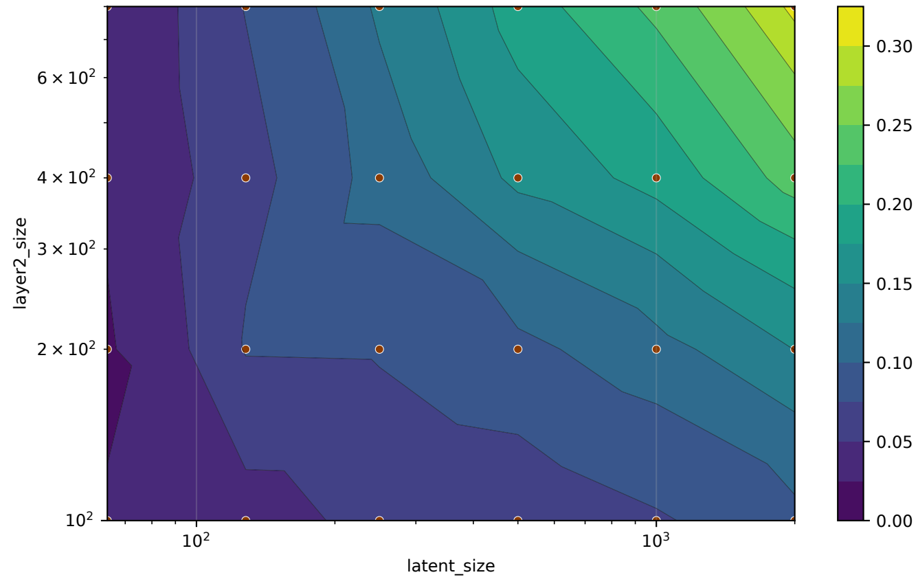
train/sparsity_rate (steps=start..2000, last)
