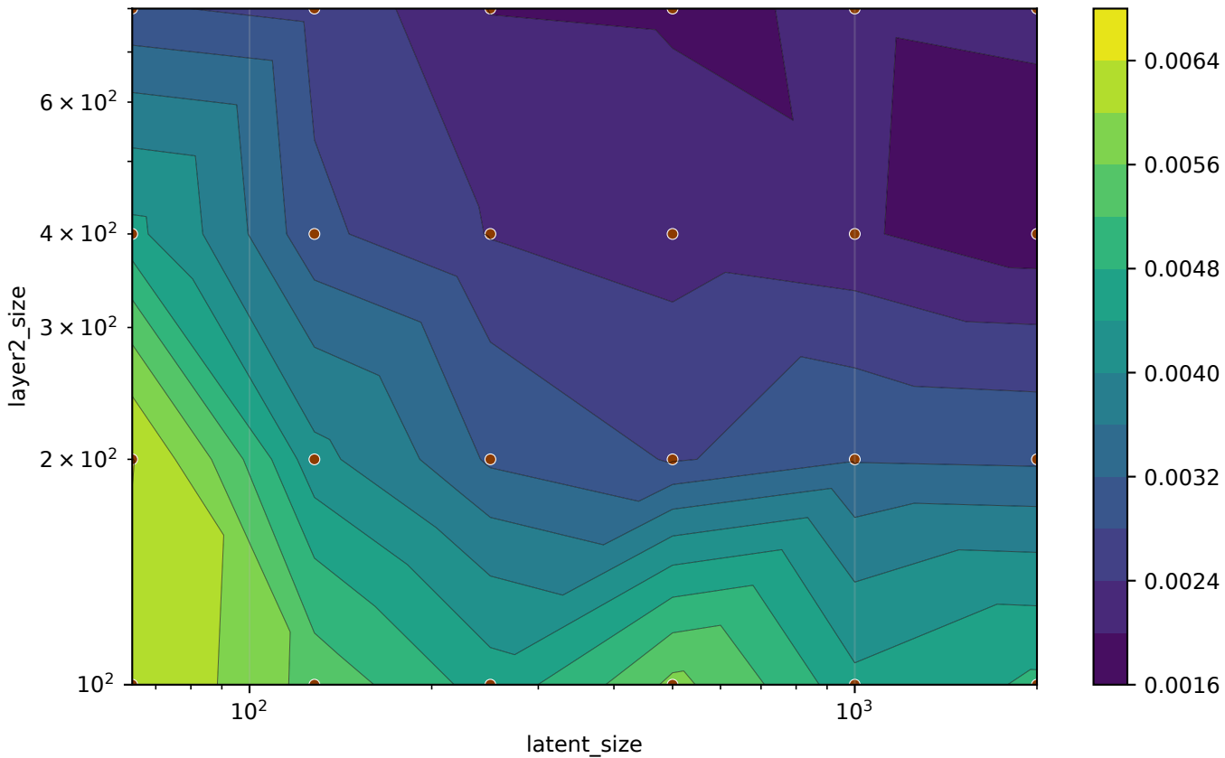
hp_metric (steps=all, last)
