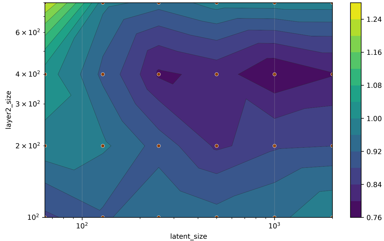
val/h1_alignment (steps=all, last)
