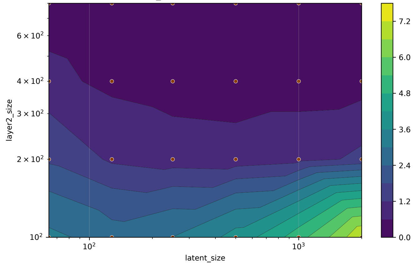
val/h2_alignment (steps=all, last)
