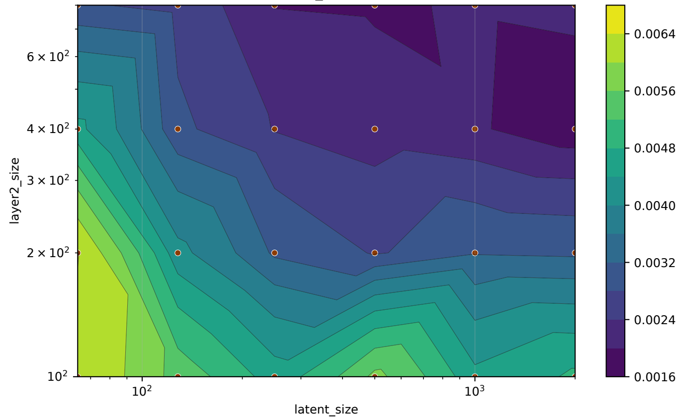
val/reconstruction_bce (steps=all, last)
