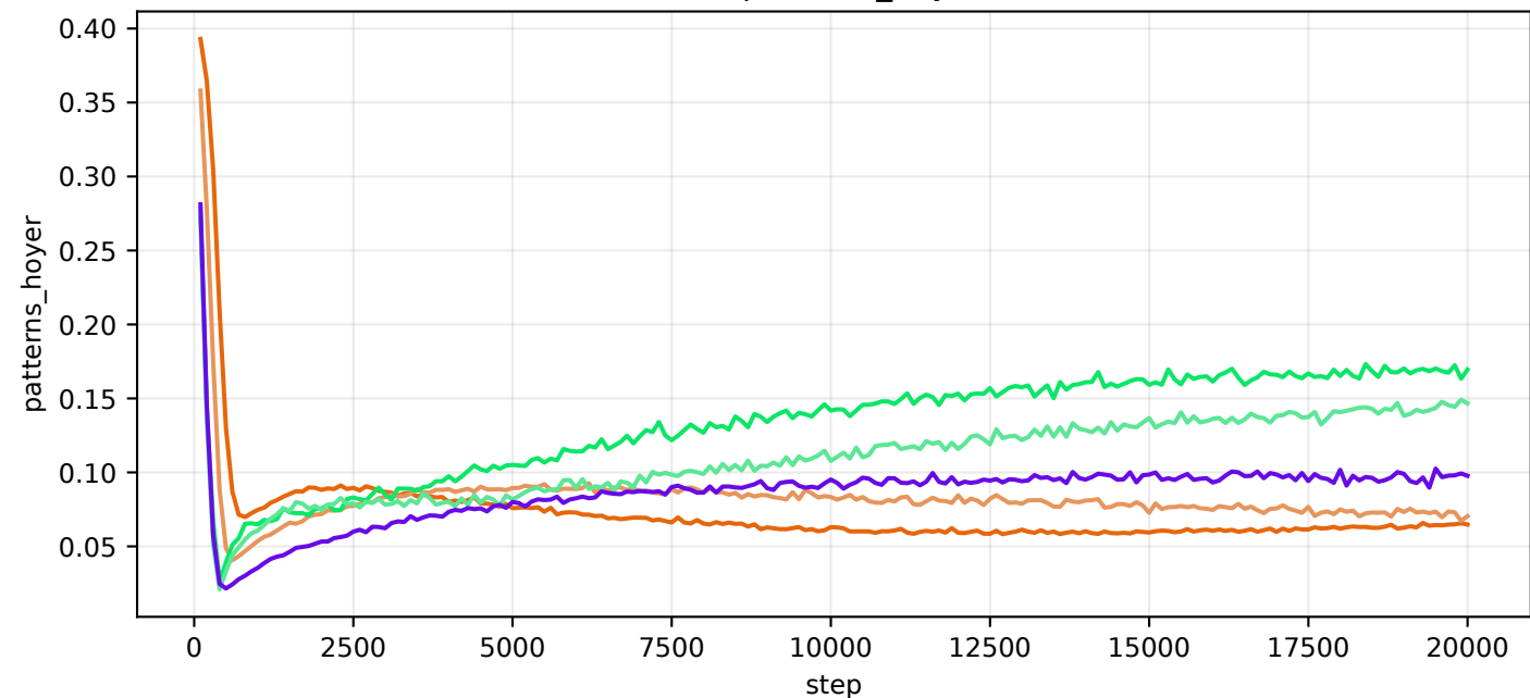
val/patterns_hoyer
