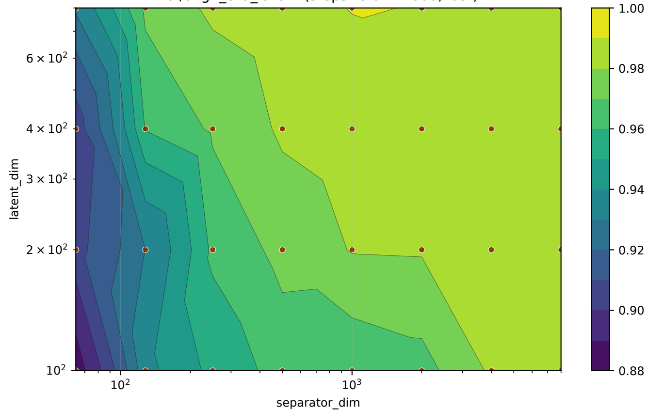
val/align_cka_latent (steps=start..2000, last)
