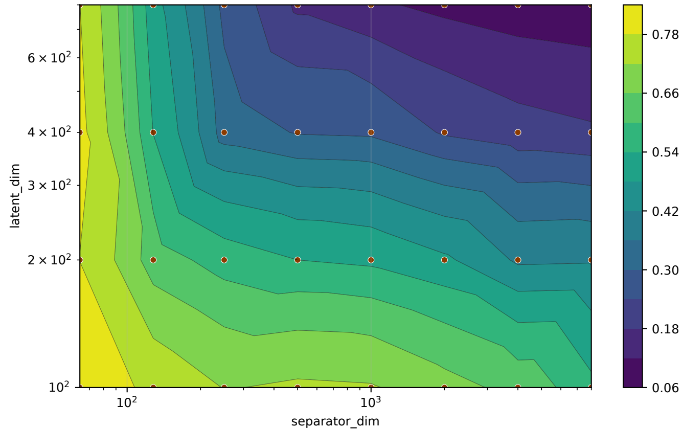
val/patterns_corr_offdiag (steps=start..2000, last)
