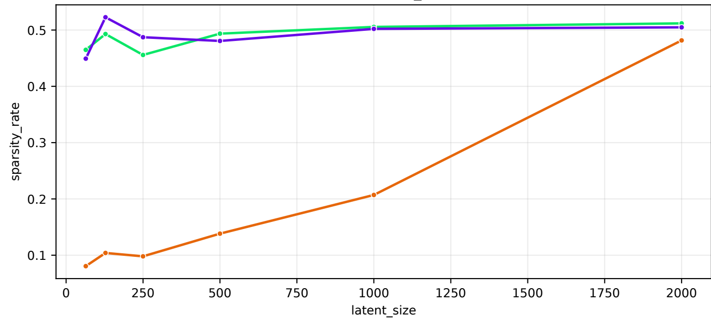
train/sparsity_rate
