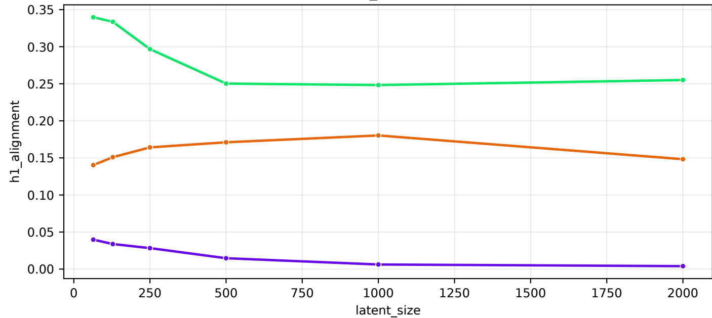
val/h1_alignment
