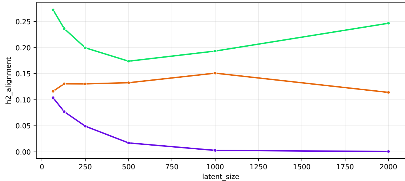
val/h2_alignment
