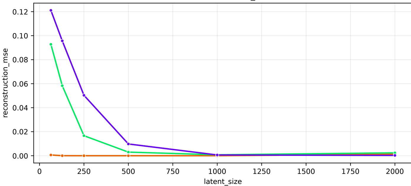
val/reconstruction_mse
