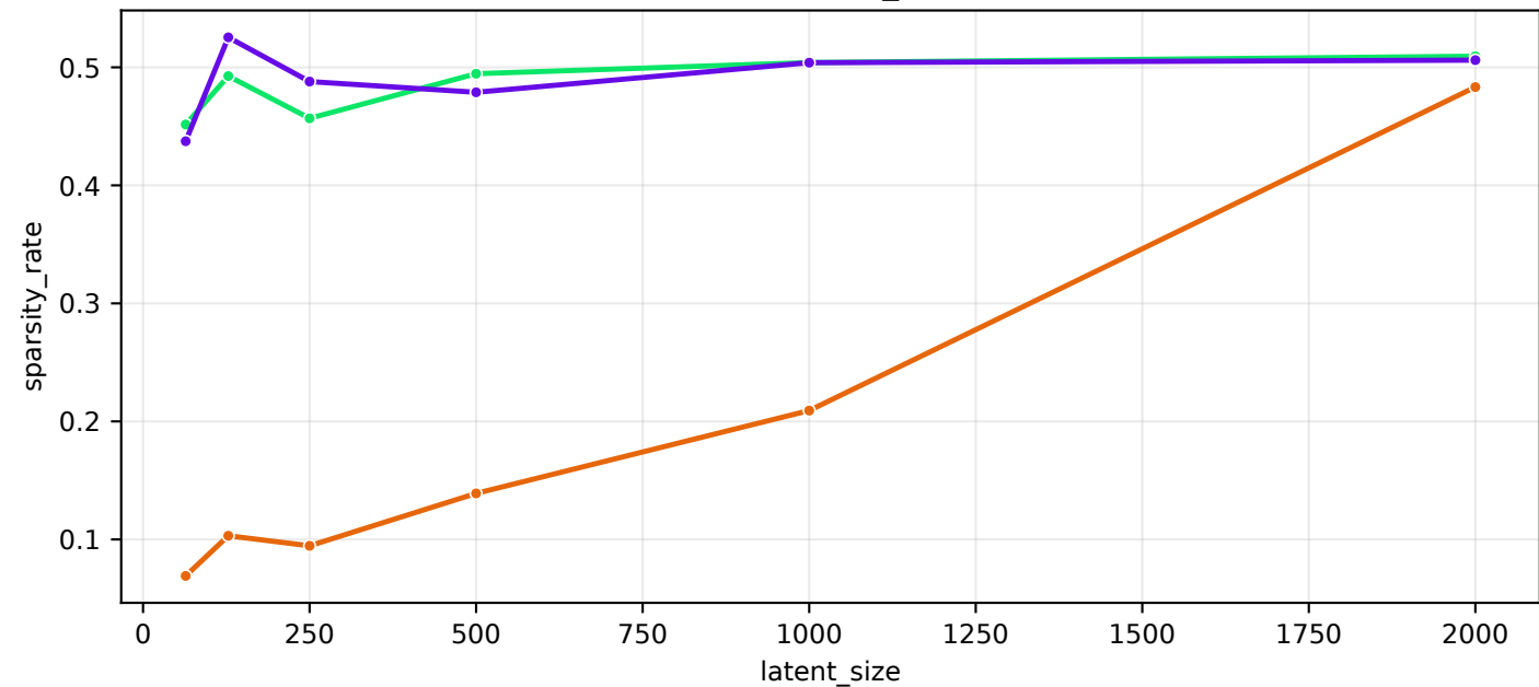
val/sparsity_rate
