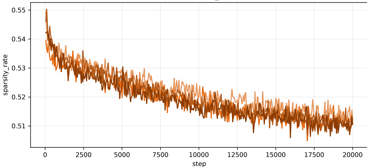
train/sparsity_rate
