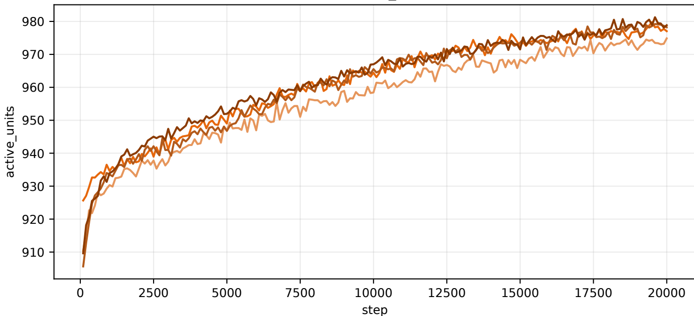
val/active_units
